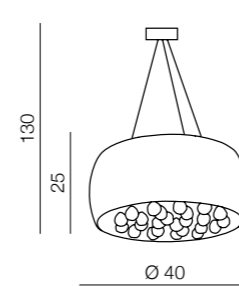
Caldo 40 AZ1002 5x G9 Only LED metal/chrome/glass
