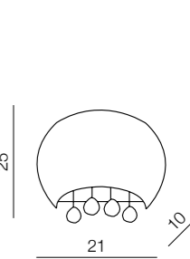
Caldo wall AZ1004 1x G9 Only LED metal/chrome/glass
