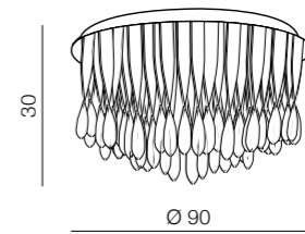
Jewel 90 AZ1661 (chrome) G9 10x MAX 40W aluminium
