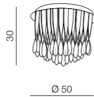
Jewel 50 AZ1663 (chrome) G9 7x MAX 40W aluminium
