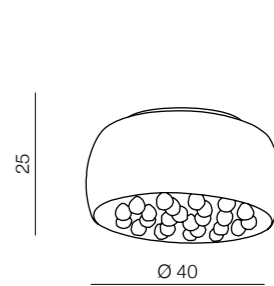
Caldo 40 top AZ1002 6x G9 Only LED metal/chrome/glass
